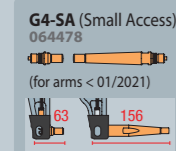
G4-SA (Small Access) 064478 (for arms < 01/2021)
