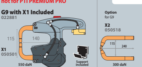
G9 with X1 Included 022881
